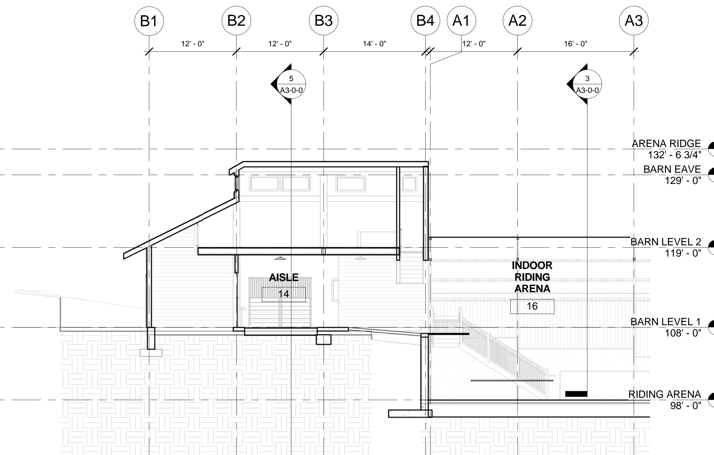
4 BUILDING SECTION 4 1/8" = 1'-0"
