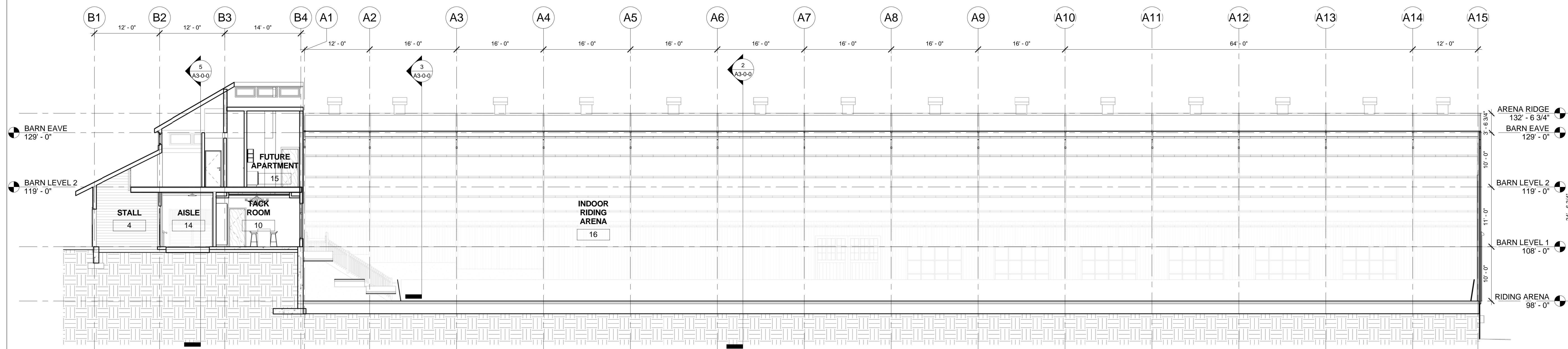
1 BUILDING SECTION 1 1/8" = 1'-0"
