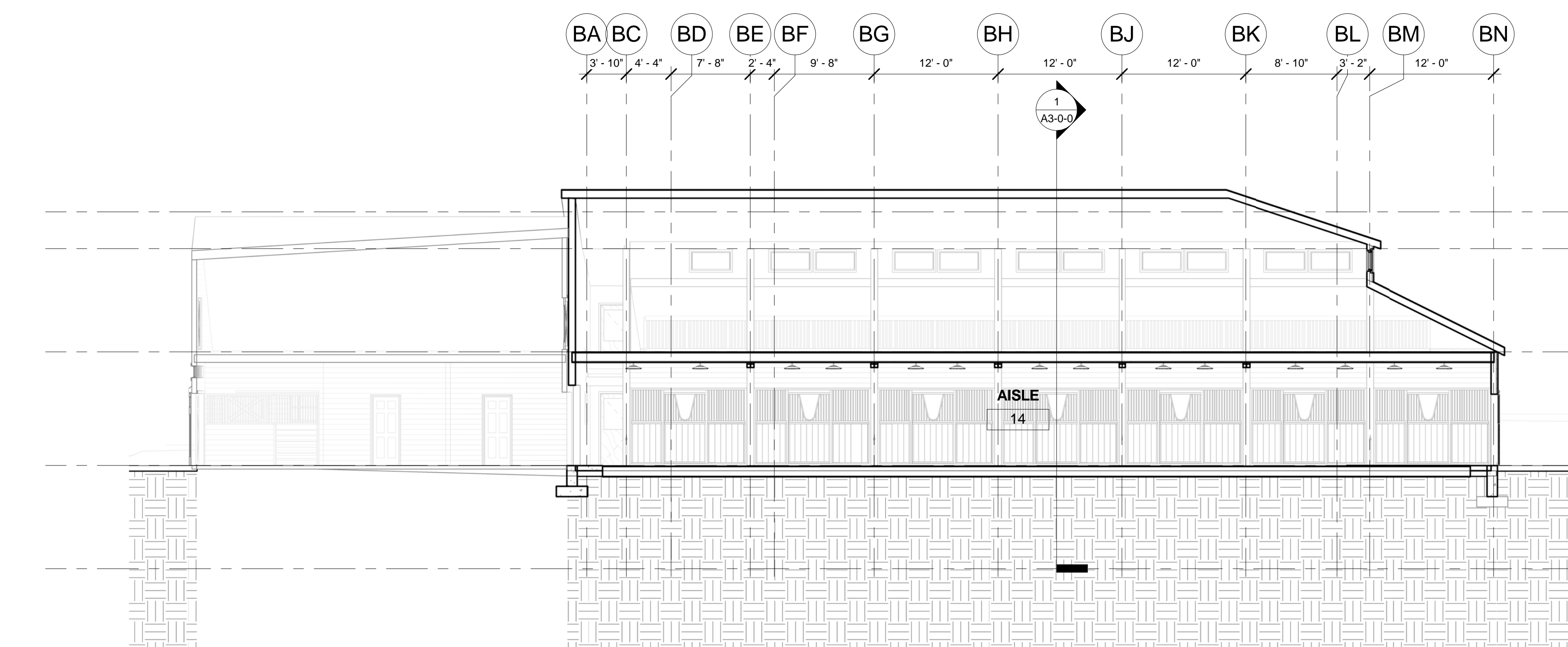
5 BUILDING SECTION 5 1/8" = 1'-0"
