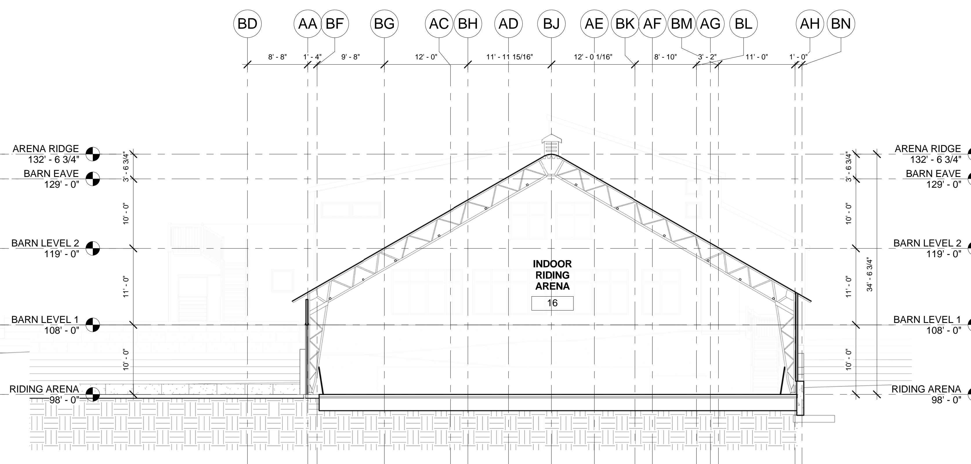
2 BUILDING SECTION 2 1/8" = 1'-0"
