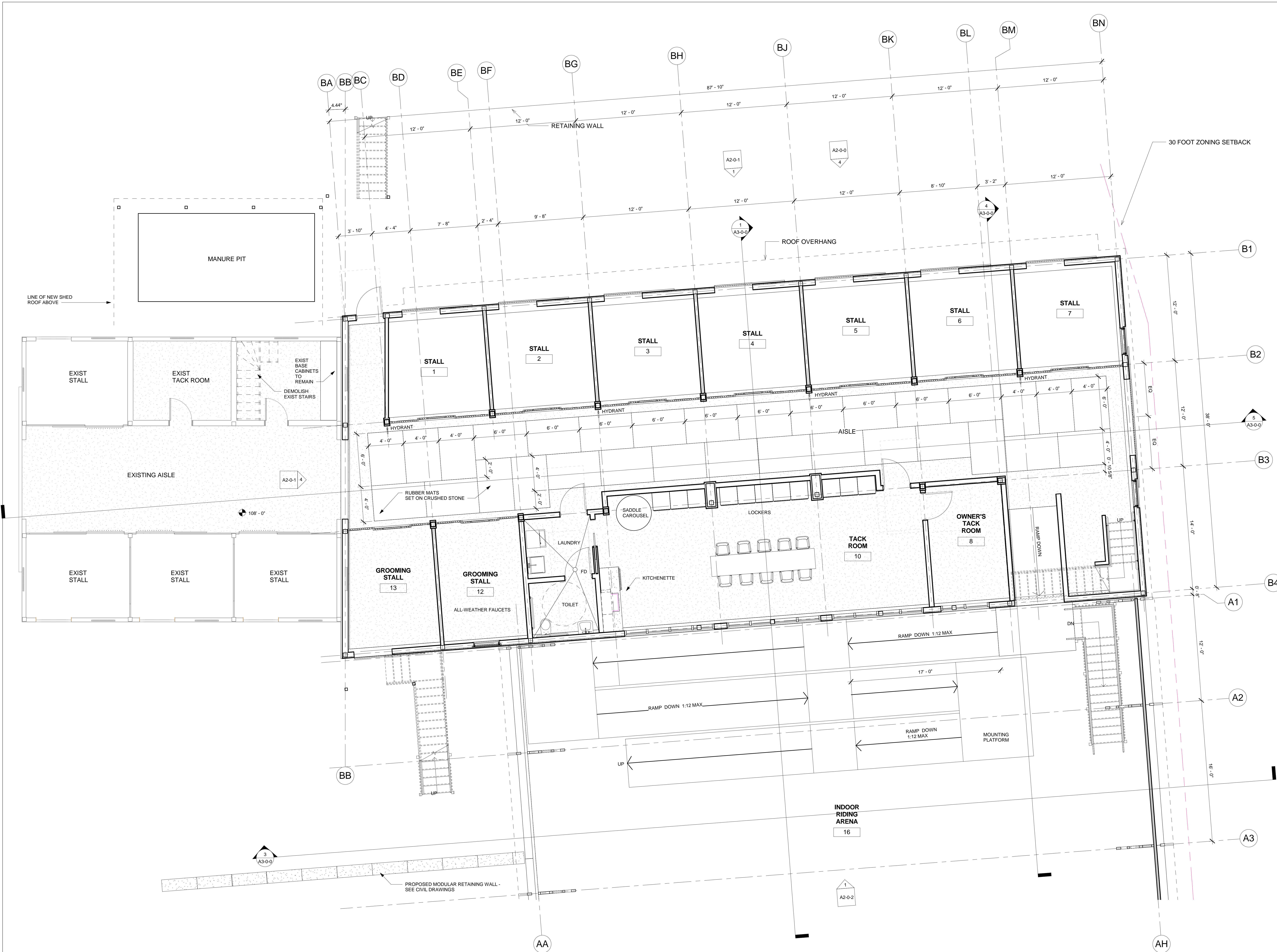
1 BARN LEVEL 1 - ENLARGED 1/4" = 1'-0"
